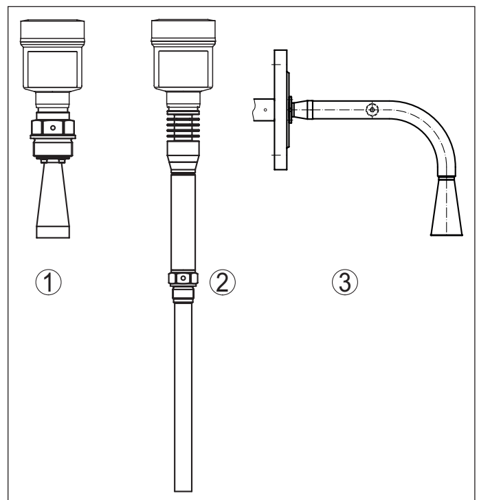
Fig. 4: Antenna systems VEGAPULS 6X for special applications
