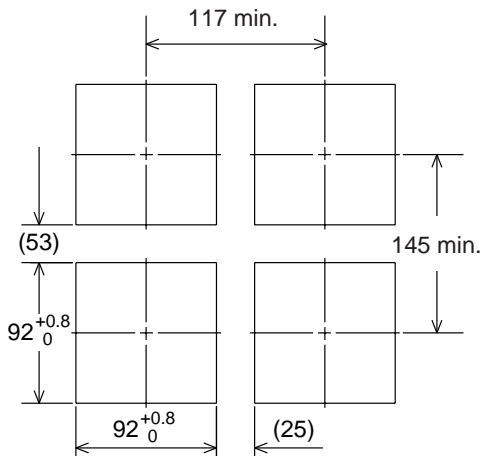
General installation
