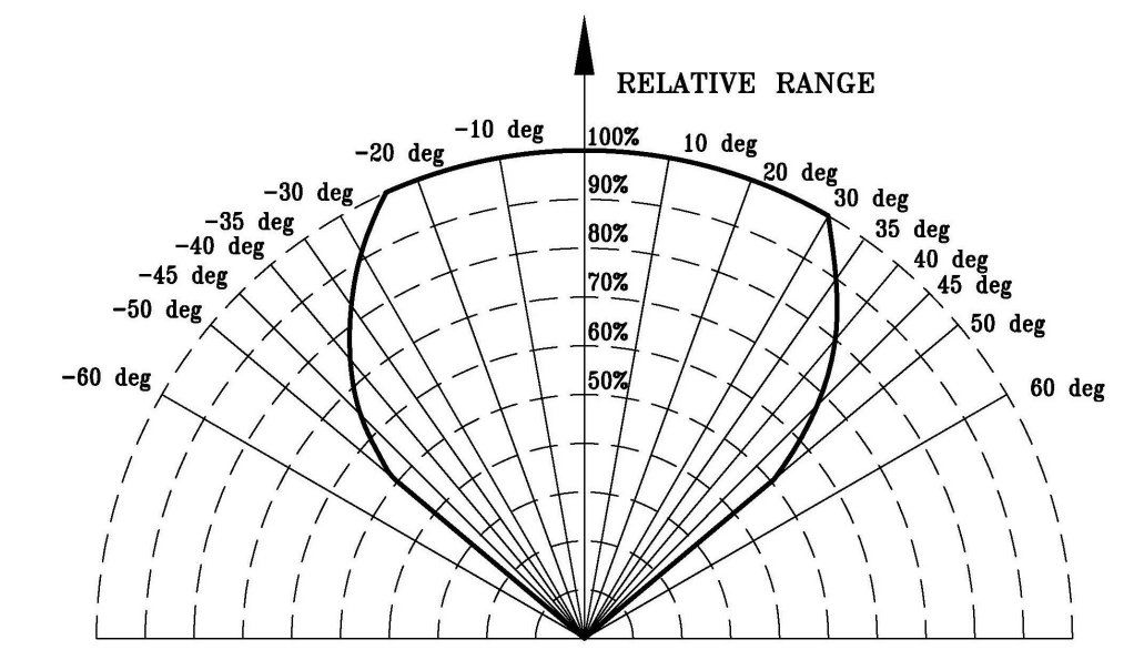
Figure 2-1: Horizontal field of view for Rosemount 975MR
