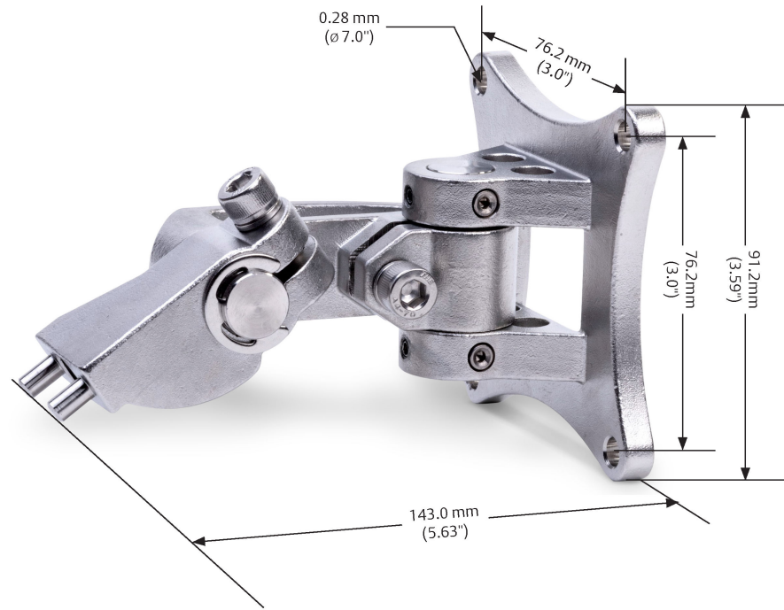
Figure 2-15: Tilt mount
