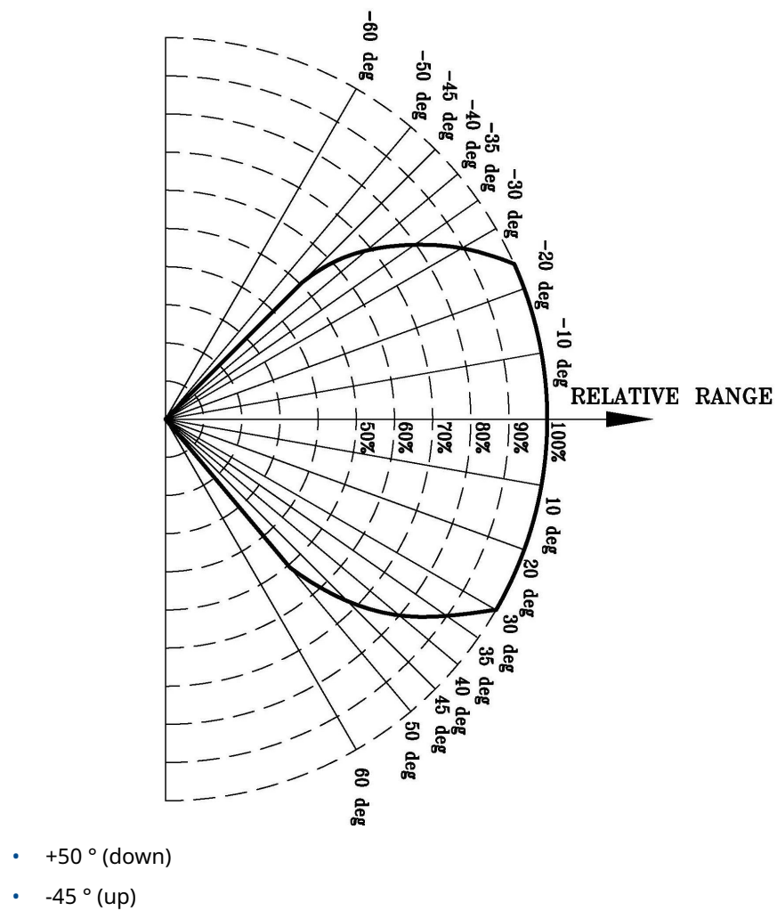
Figure 2-2: Vertical field of view for Rosemount 975MR
