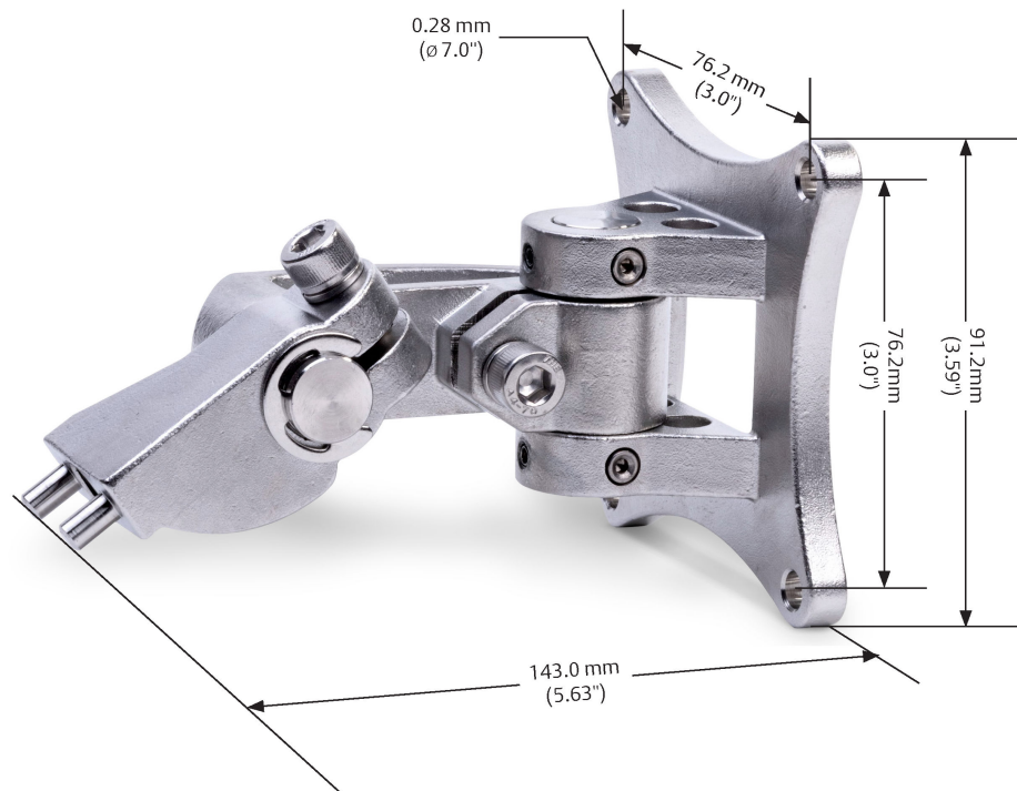
Figure 2-9: Tilt mount with dimensions
