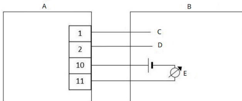
Figure 2-13: Sink four-wire
