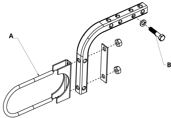
Figure 4: "L" Bracket Exploded View
