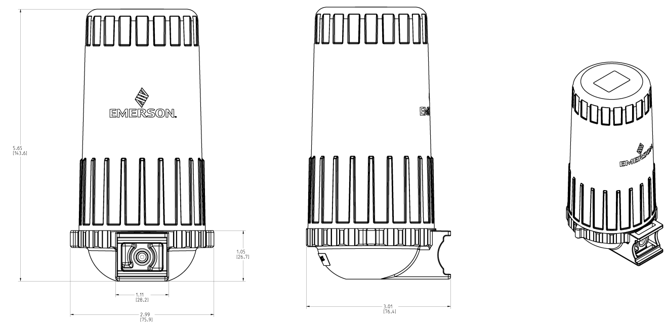
Figure 2: Rosemount Synchros™ WirelessHART® Repeater Dimensions
