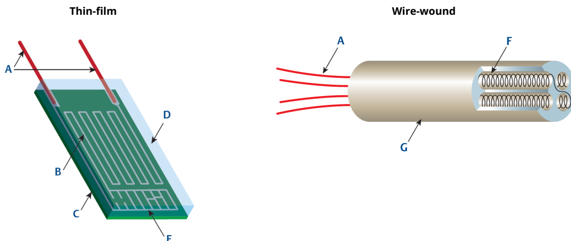
Figure 3: RTD Elements
