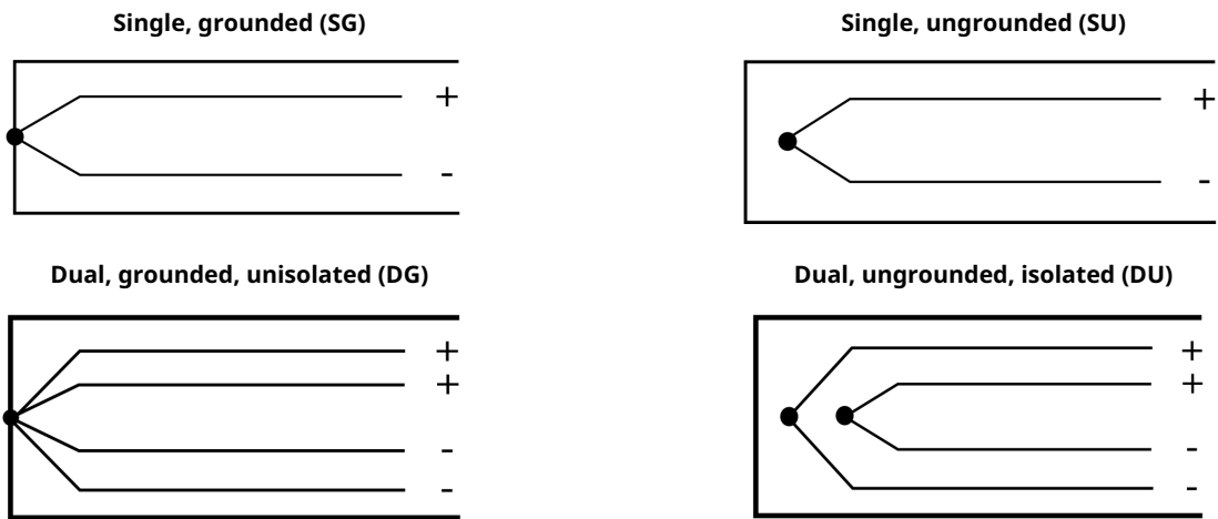
Figure 12: Thermocouple Lead Wire Configurations
