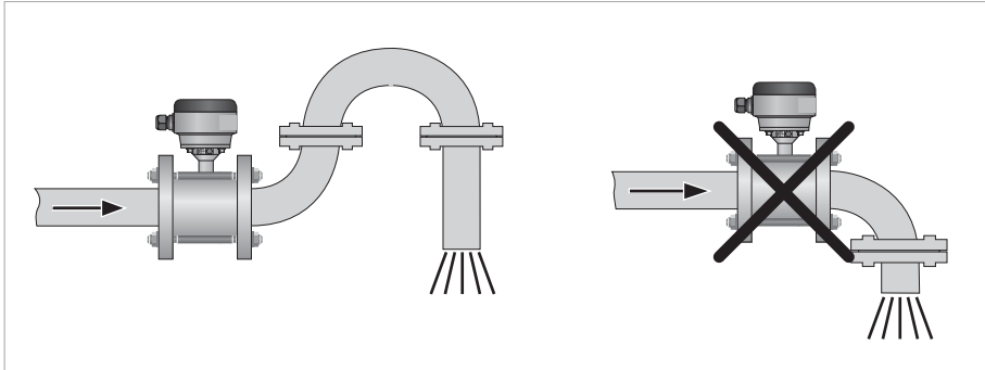
Figure 3-7: Installation in front of an open discharge
