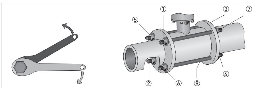
Figure 3-14: Tighten the bolts in fixed order, see picture.
