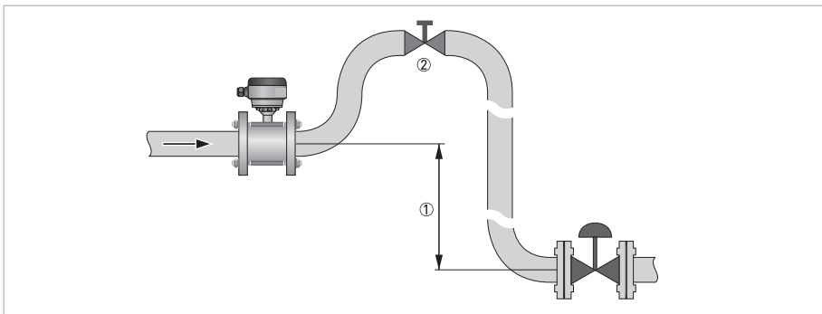
Figure 3-11: Air venting
