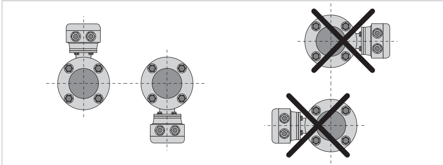
Figure 3-13: Mounting position
