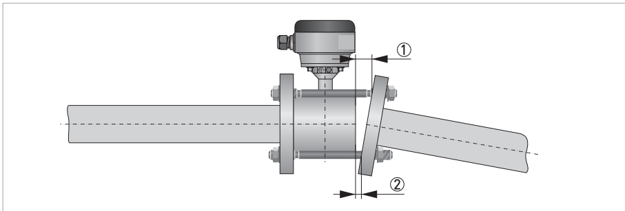
Figure 3-8: Flange deviation
