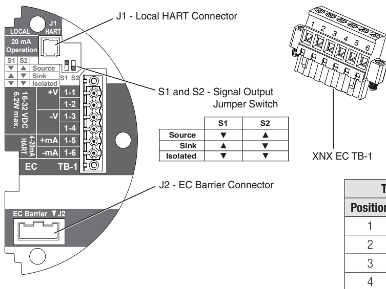
Figure 9. XNX EC personality board terminal blocks, jumper switches, and terminal block assignments
