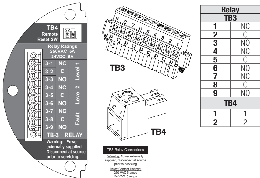
Figure 24. XNX relay option board and terminal block
