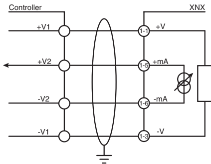
Figure 7. Isolated wiring for XNX
