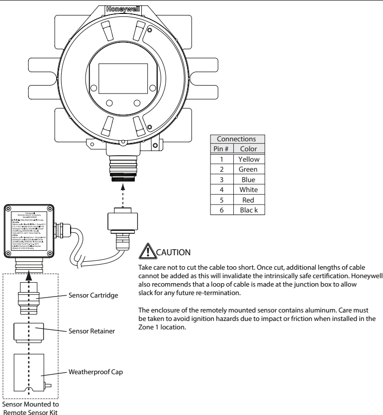
Figure 12. Installing remote sensor mounting kit
