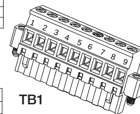
Figure 49. IR personality board terminal blocks, jumper switches and wiring guide
