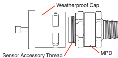
Figure 3. MPD, Adaptor and Weatherproof Cap
