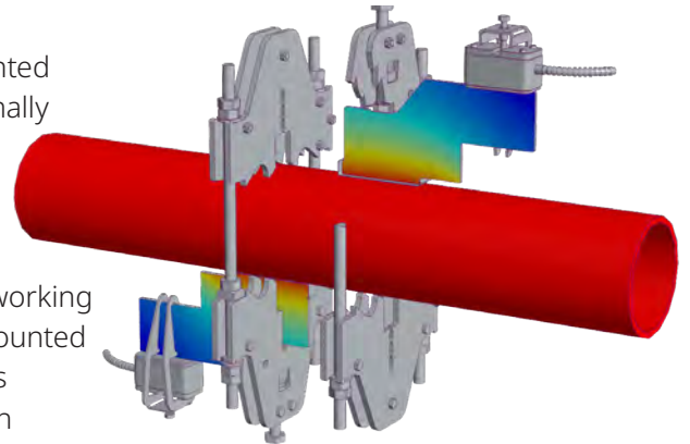
Temperature profile of the WaveInjector®
