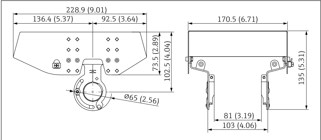
53 Dimensions. Unit of measurement mm (in)
