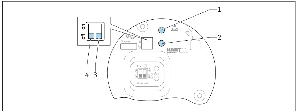
51 Operating keys and DIP switches on the HART electronic insert
