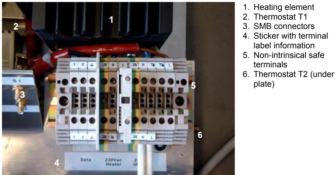
Figure 1: Non-intrinsically safe terminals of UFC-V/LT-EEx
