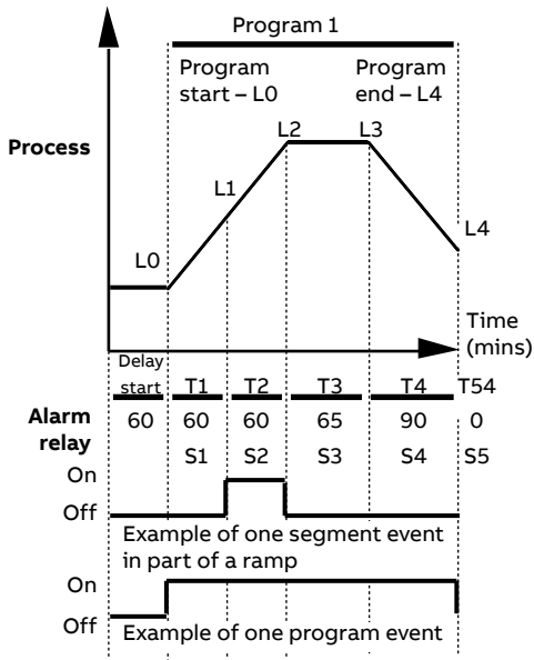
02 Ramp/Soak program with time event relay sequences
