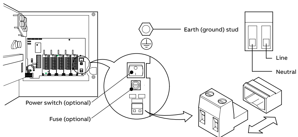
O8 Power supply connections
