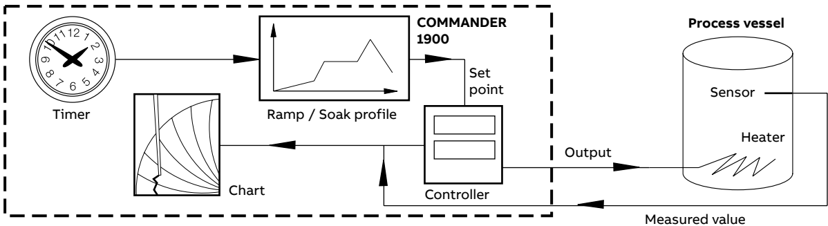
03 Programmed process warm-up triggered by real-time clock
