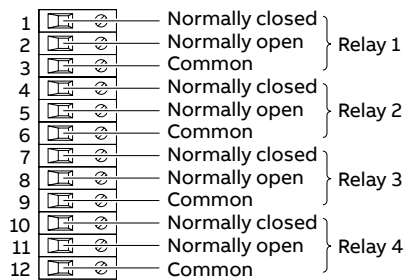
O6 4-relay output module
