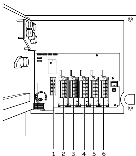
09 Module positions
