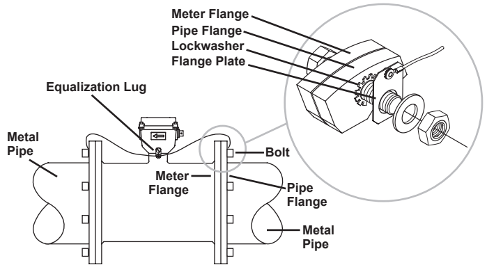
Equalization Diagram
