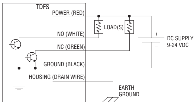
FIGURE 3: Wiring Diagram
