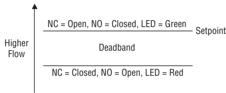
FIGURE 1: Switch Setpoint & Deadband
