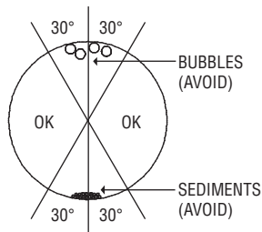
FIGURE 2: Mounting Orientation
