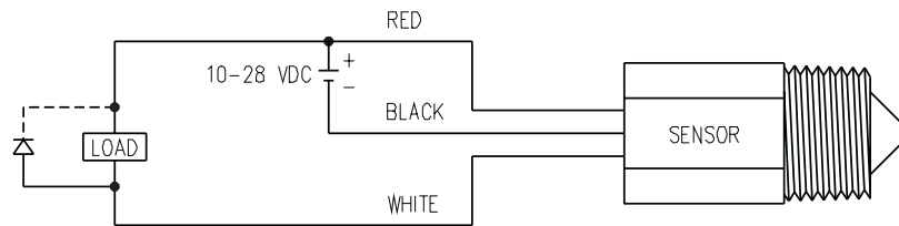
EXTERNAL LOAD WITH 1 SUPPLY
