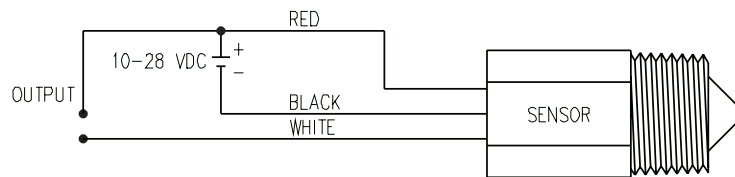
OPEN COLLECTOR OUTPUT
