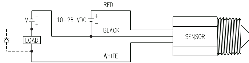
EXTERNAL LOAD WITH 2 SUPPLIES
