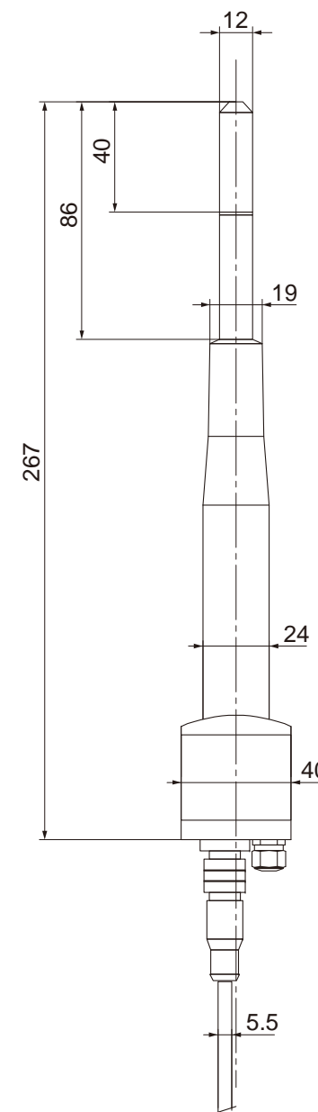
Figure 3 HMP155
