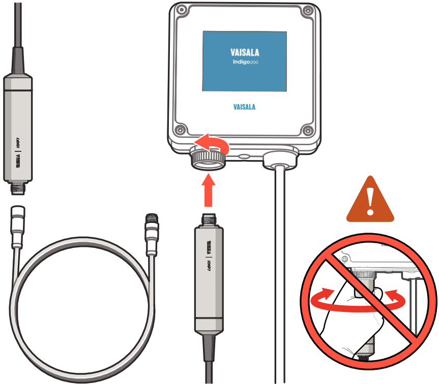
Figure 15 Attaching the Probe to Indigo 200 Series
