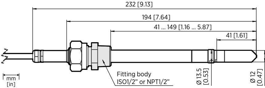
Figure 31 HMP8 Probe Head Dimensions
