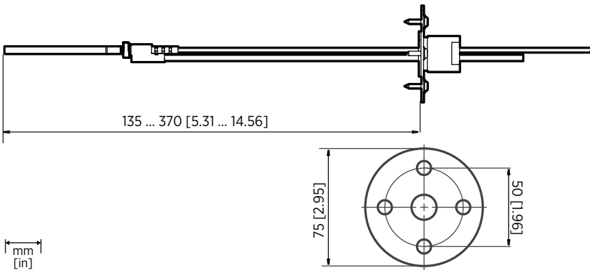
Figure 33 Optional Duct Kit 215003 Dimensions
