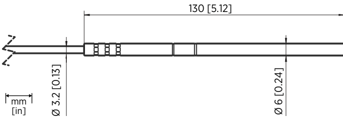
Figure 32 TMP1 Probe Head Dimensions
