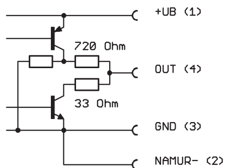
Push Pull + NAMUR
