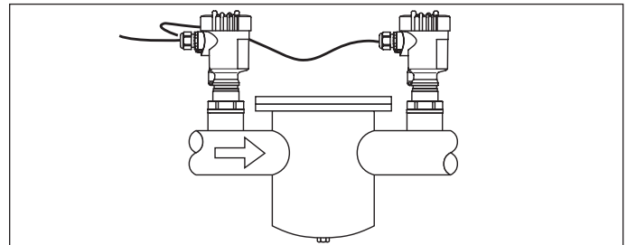
Fig. 13: Electronic differential pressure measurement through Master/Slave combination
