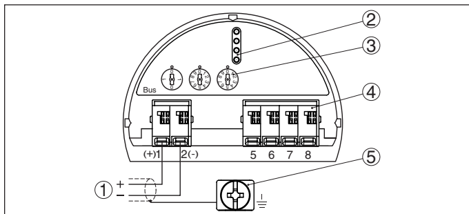
Fig. 28: Electronics and connection compartment, single chamber housing
