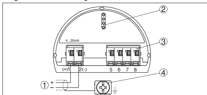
Fig. 26: Electronics and connection compartment, single chamber housing
