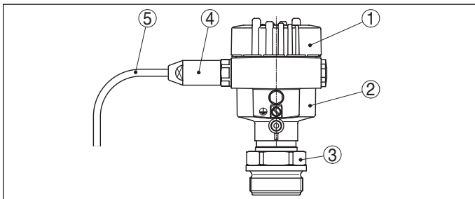
Fig. 10: Example of a VEGABAR 82 with aluminium housing in protection class IP 68, 1 bar
