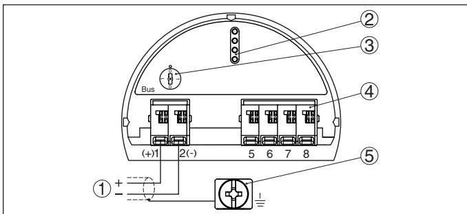
Fig. 30: Electronics and connection compartment, single chamber housing
