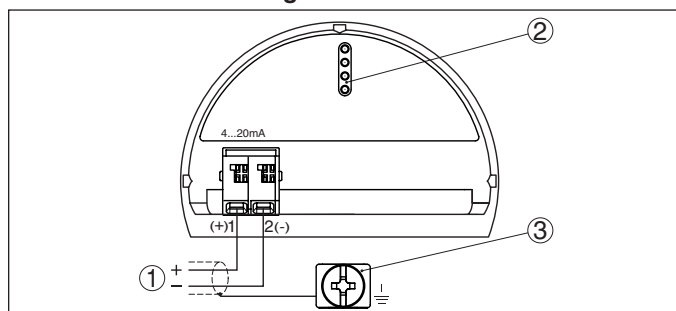
Fig. 27: Connection compartment, double chamber housing
