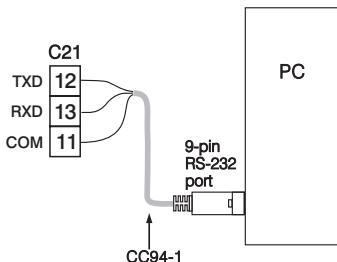
Figure 2.22 RS-232 Wiring
