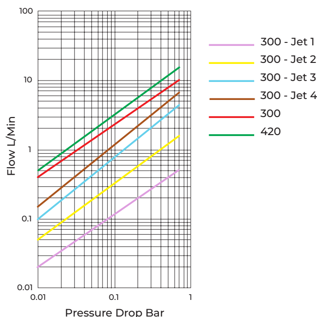
Pressure Drop vs. Flow Rate
