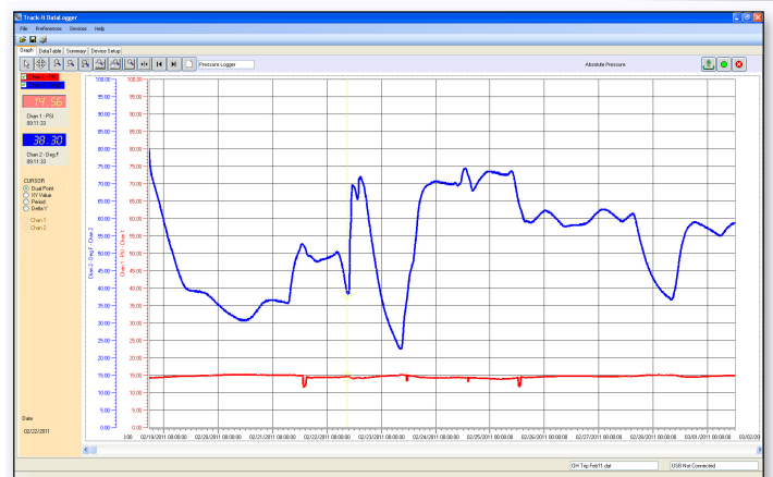
Track-It™ Software
