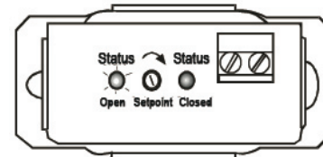
Figure 9: Status Open, LED On
