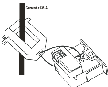
Figure 4: CSC with CT Transformer
