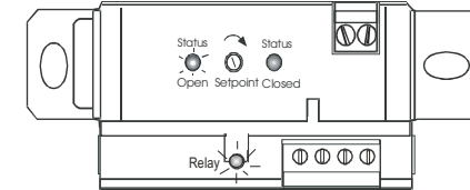
Figure 8: Status Open, LED On
