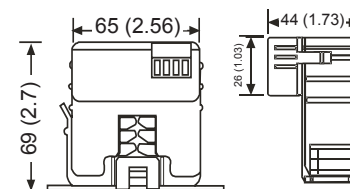
Figure 1: CSC Dimensions mm (in.)
