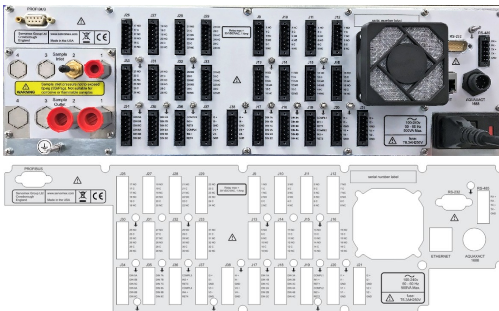
Figure 3-4: Rear of 4900 Multigas
