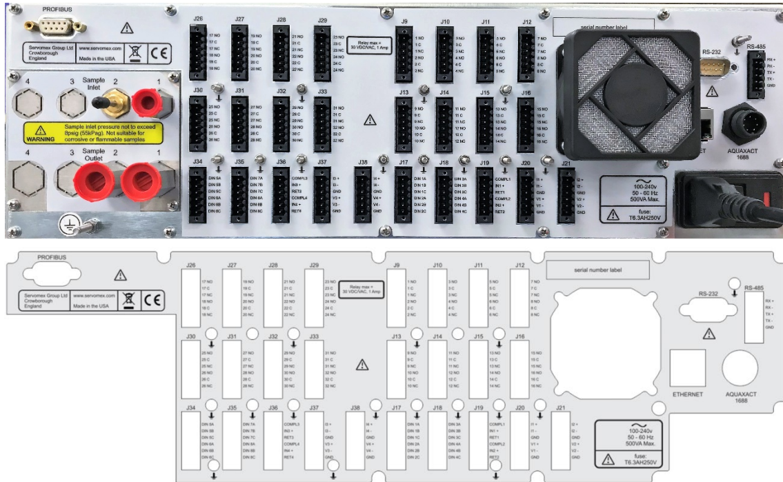
Figure 2-1: Rear of the 4900 Multigas analyzer
