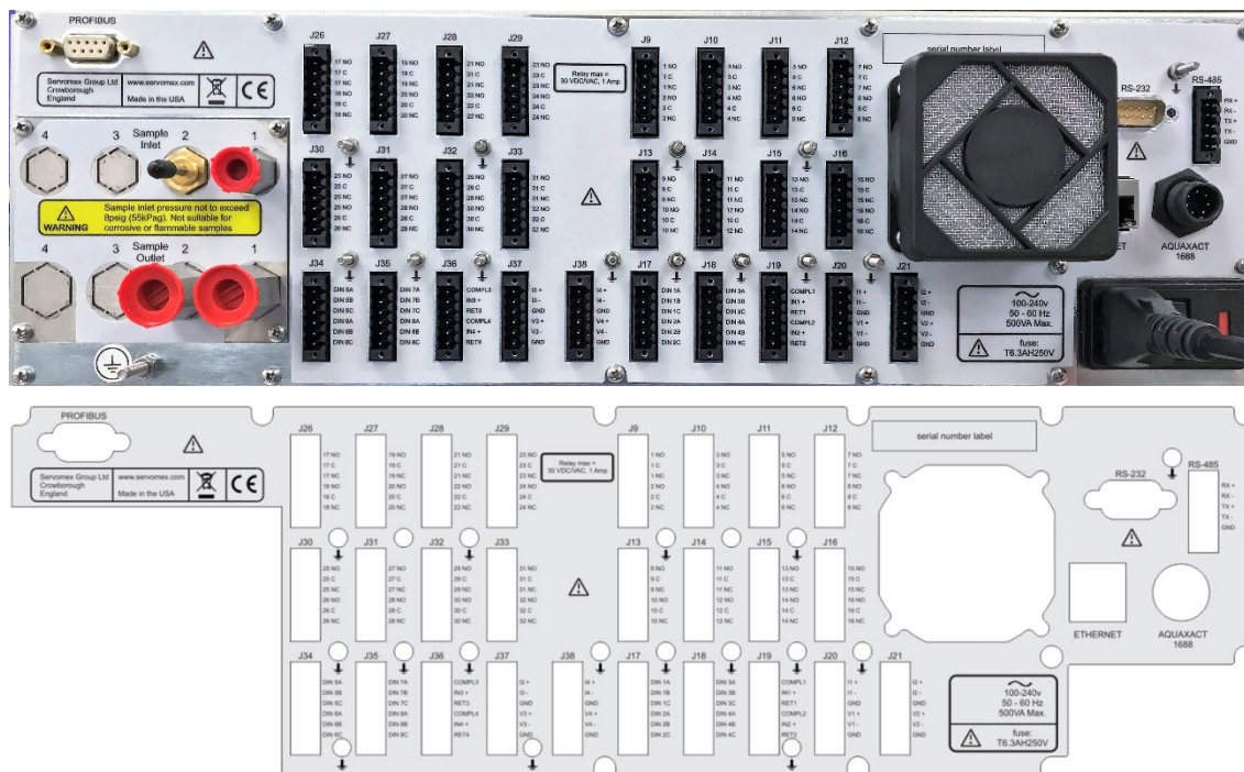
Figure 1-2: Rear of the 4900 Multigas Gas Analyzer configured for use with an external NO 2 Converter (two inlet / outlet lines included)
