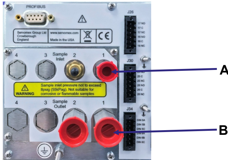
Figure 3-6: Gas inlets and outlets on rear of analyzer – Standard systems use Sample Inlet / Outlet #1 only.
