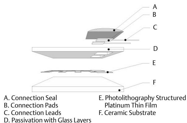
Figure 7. Construction of a Platinum Thin Film RTD
