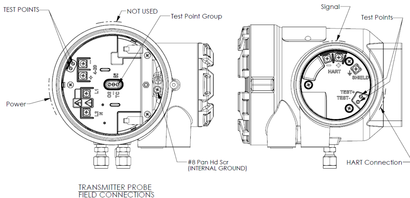
Figure 4. Rosemount 6888A with Autocalibration Housing Field Connections - HART Output
