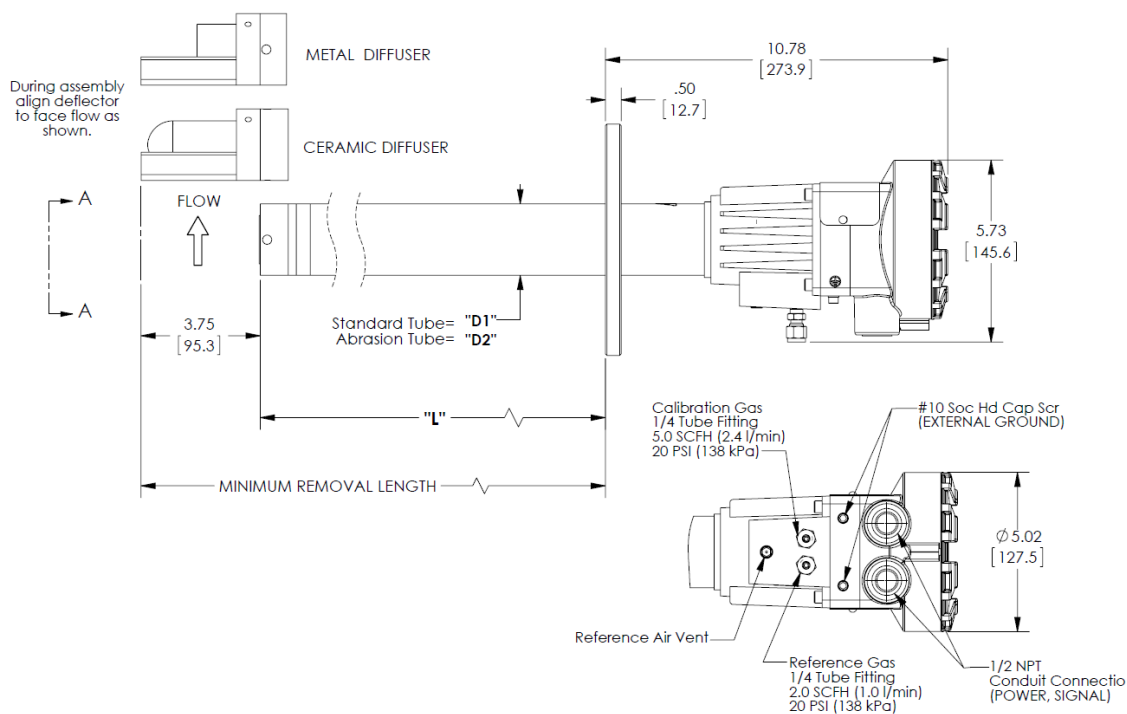
Figure 2. Rosemount™ 6888A with Standard Housing
