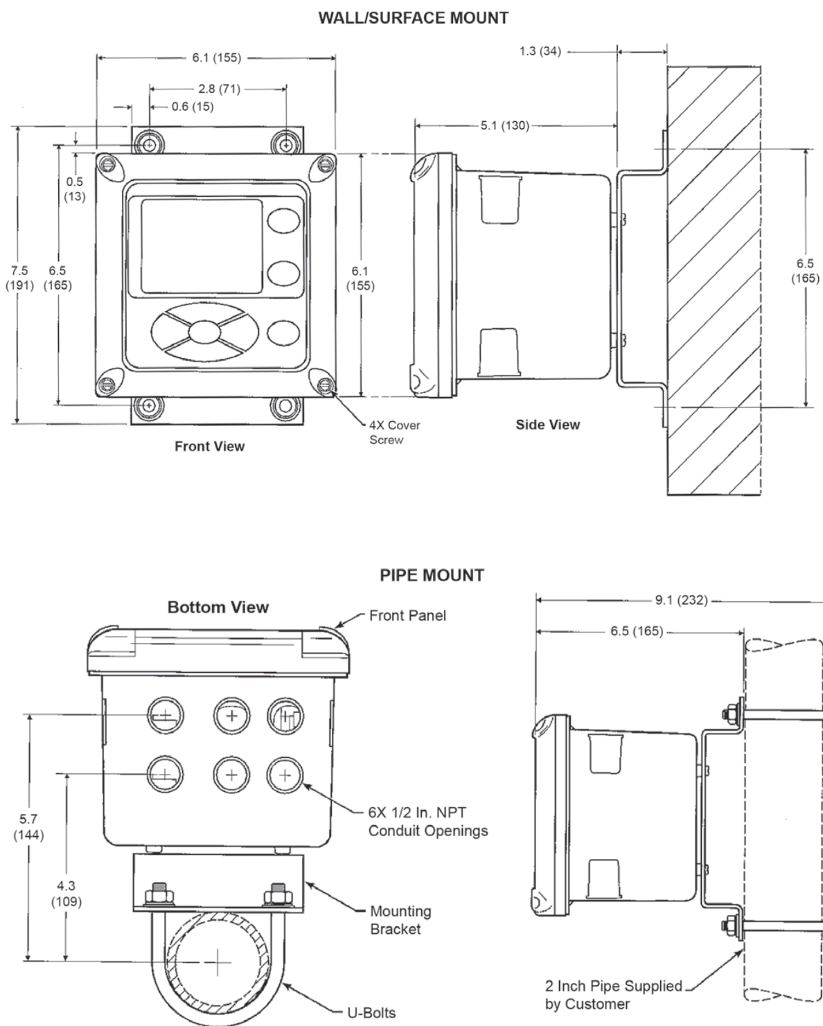
Figure 12. Rosemount 6888 Xi with Wall/Pipe Mount
