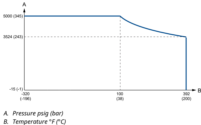
Figure 17: C - Cryogenic Temperature Tank Connection (Code C)
