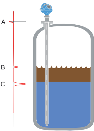
Figure 1: Measurement Principle
