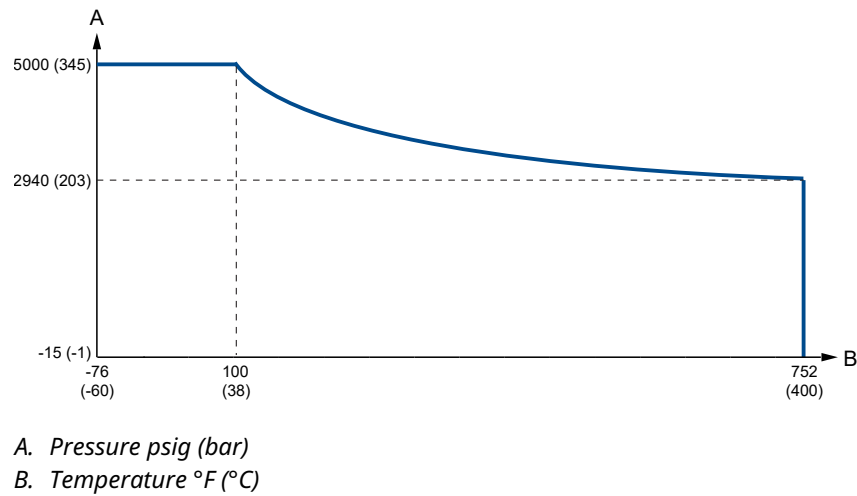
Figure 16: HP - High Pressure Tank Connection (Code P)
