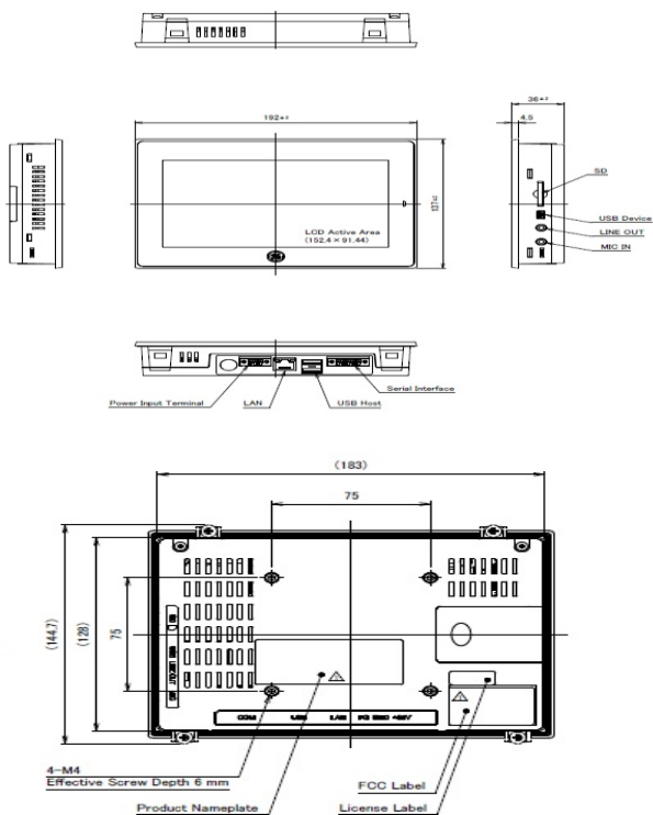
Figure 1.2: IC755CxW07CDx Profile and Hardware Features
