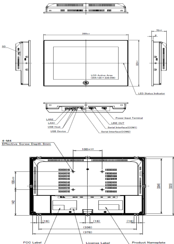
Figure 1.5: IC755CxS15CDx Profile and Hardware Features
