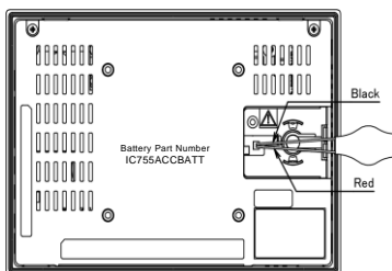
Figure 3.2: IC755CxS06RDx /IC755CxW07CDx Battery Harness Connection
