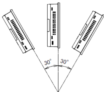
Figure 4.1: Mounting Angle
