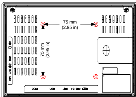
Figure 4.16: IC755CxSxxCDx VESA Mounting Holes
