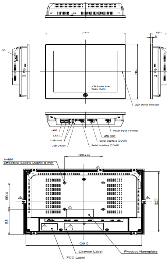
Figure 1.4: IC755CxS12CDx Profile and Hardware Features
