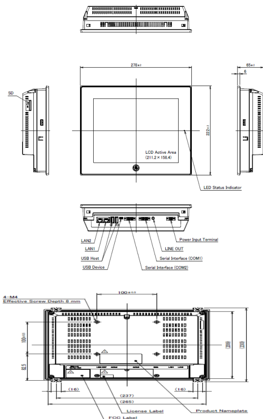
Figure 1.3: IC755CxS10CDx Profile and Hardware Features
