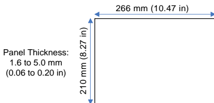
Figure 4.9: IC755CxS10CDx Panel Cutout Dimensions
