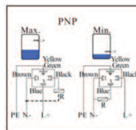
Figure 1 - PNP Output Connection Diagram
