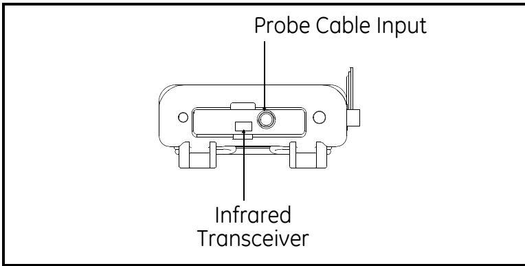
Figure 73: Probe Connection and Infrared Transceiver
