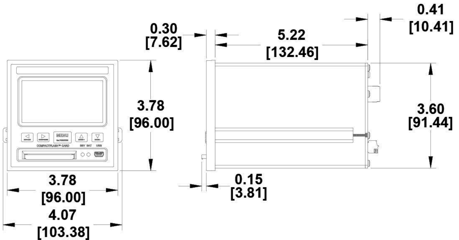
Figure 2.1 Recorder Dimensions
