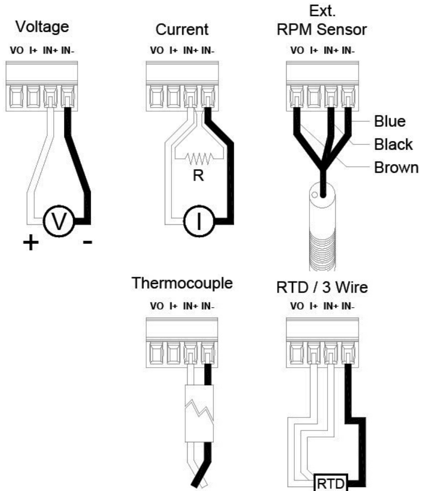
Figure 2.4 Connection Detail
