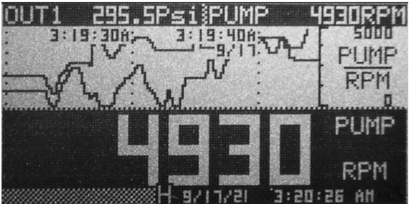
Figure 1.3 Split Screen Graphic Mode
