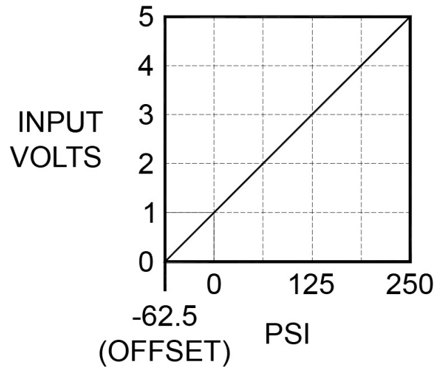
Figure 2.5 Linear Scaling
