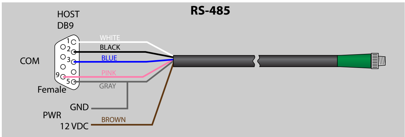
Figure 5.1.2 COM Connection Pin-out and RS-232 / RS-485 cable connections
