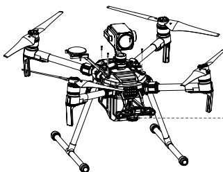
Mount the upward gimbal, and connect it to the DGC2.0 port.
