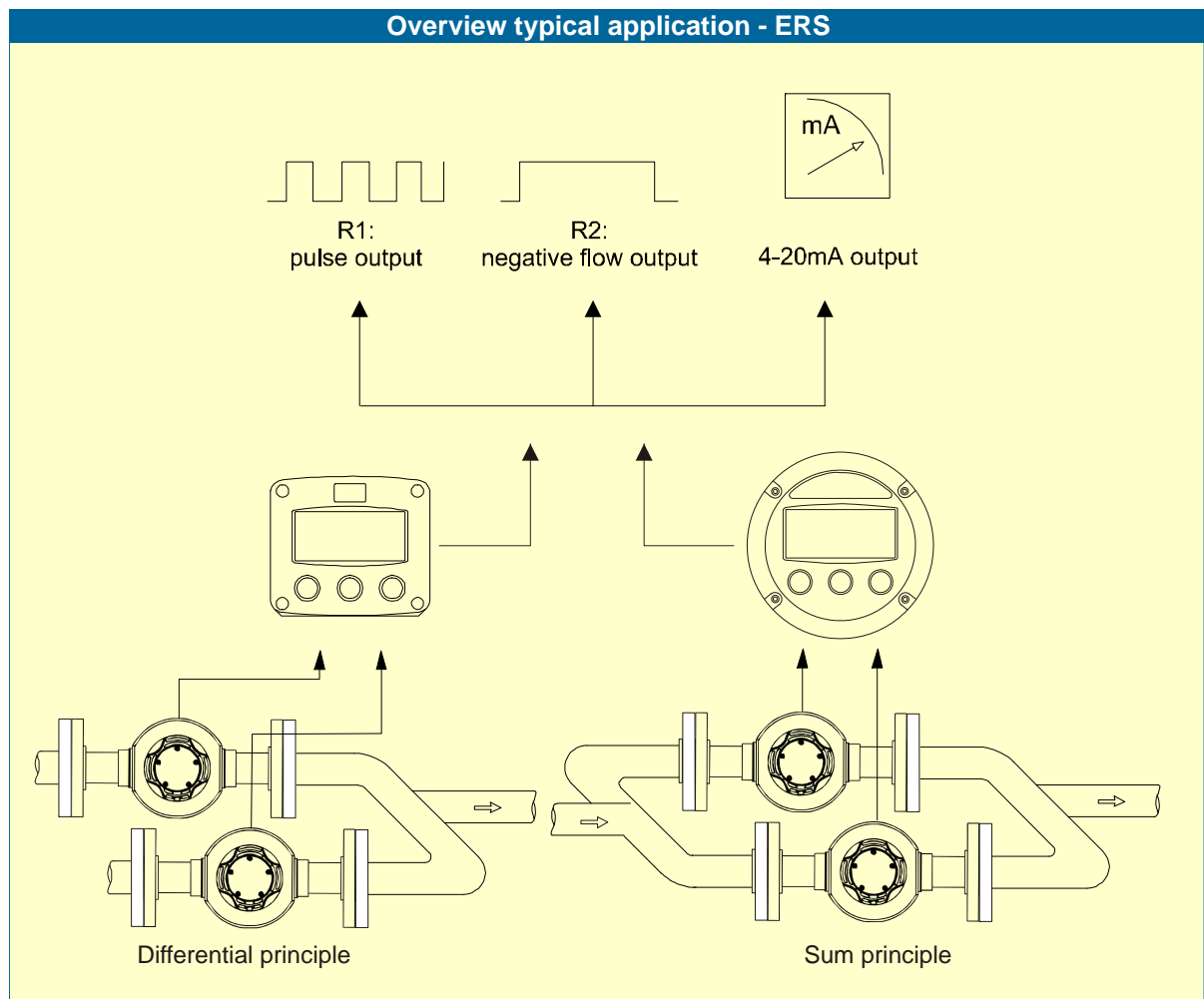
Fig. 1: Typical application for the ERS
