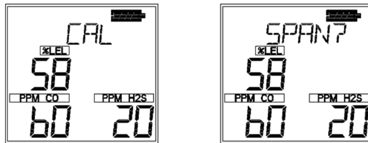
Figure 4-3. CAL Flag
