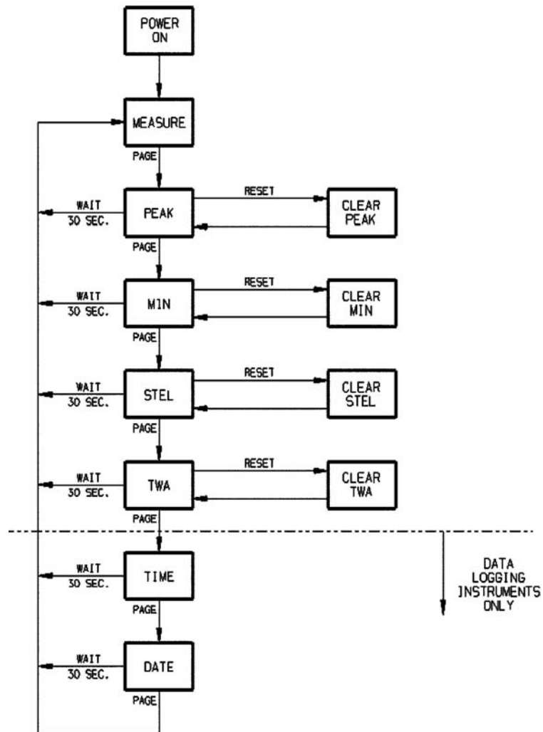
Figure 2-6. Flow Diagram
