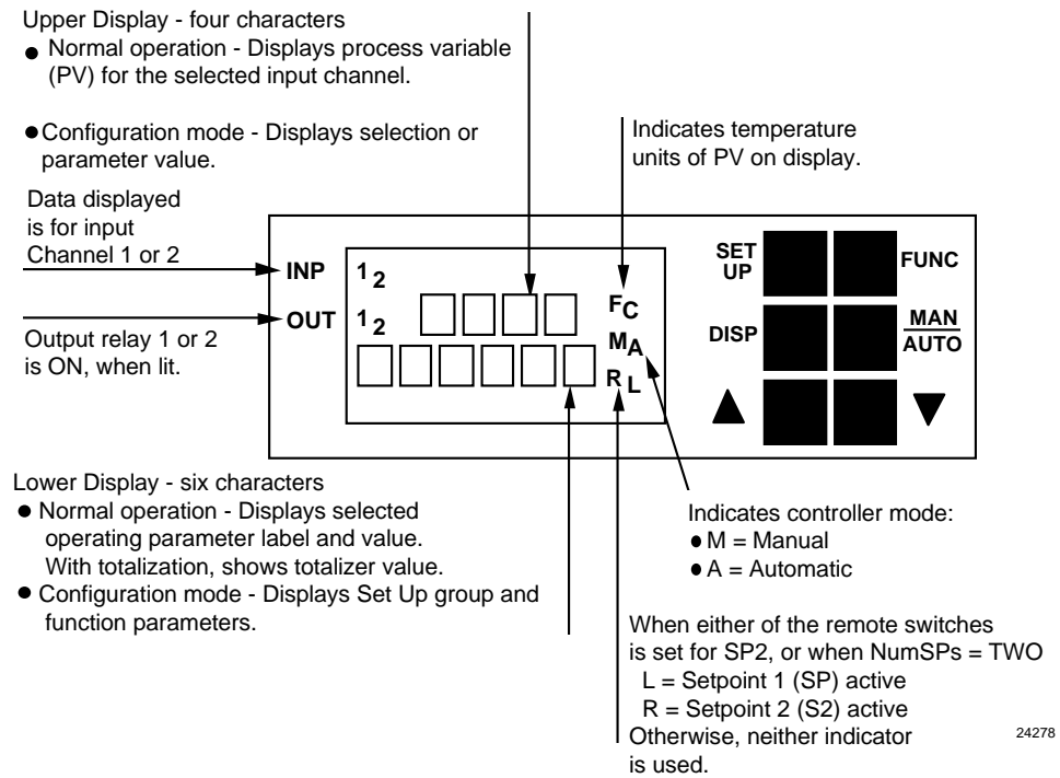
Figure 4-7 Operator Interface
