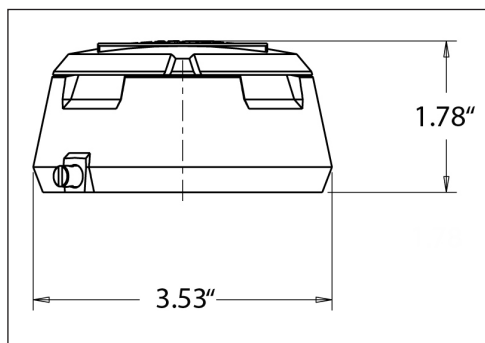
Figure 2: Front view
