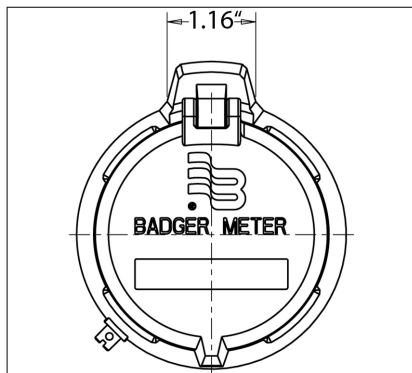
Figure 1: Top view
