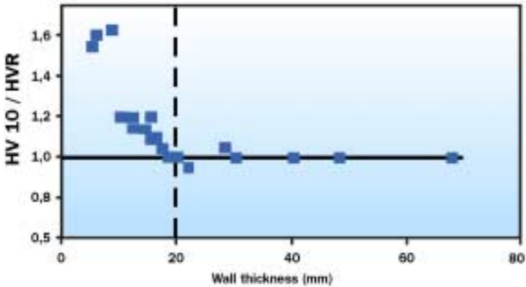
Figure 1: Comparison of HV 10 and HVR values for different wall thicknesses.
