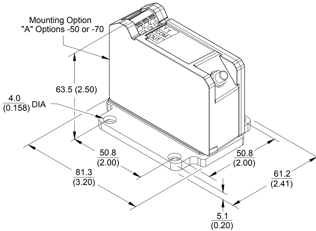
Figure 22 Panel Mount 3300 XL NSv™ Proximito® Sensor
