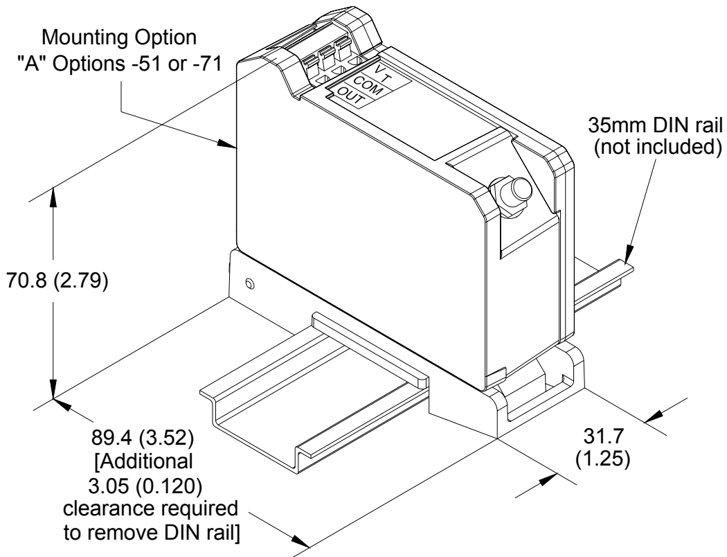
Figure 23 DIN Mount 3300 XL NSv™ Proximito® Sensor
