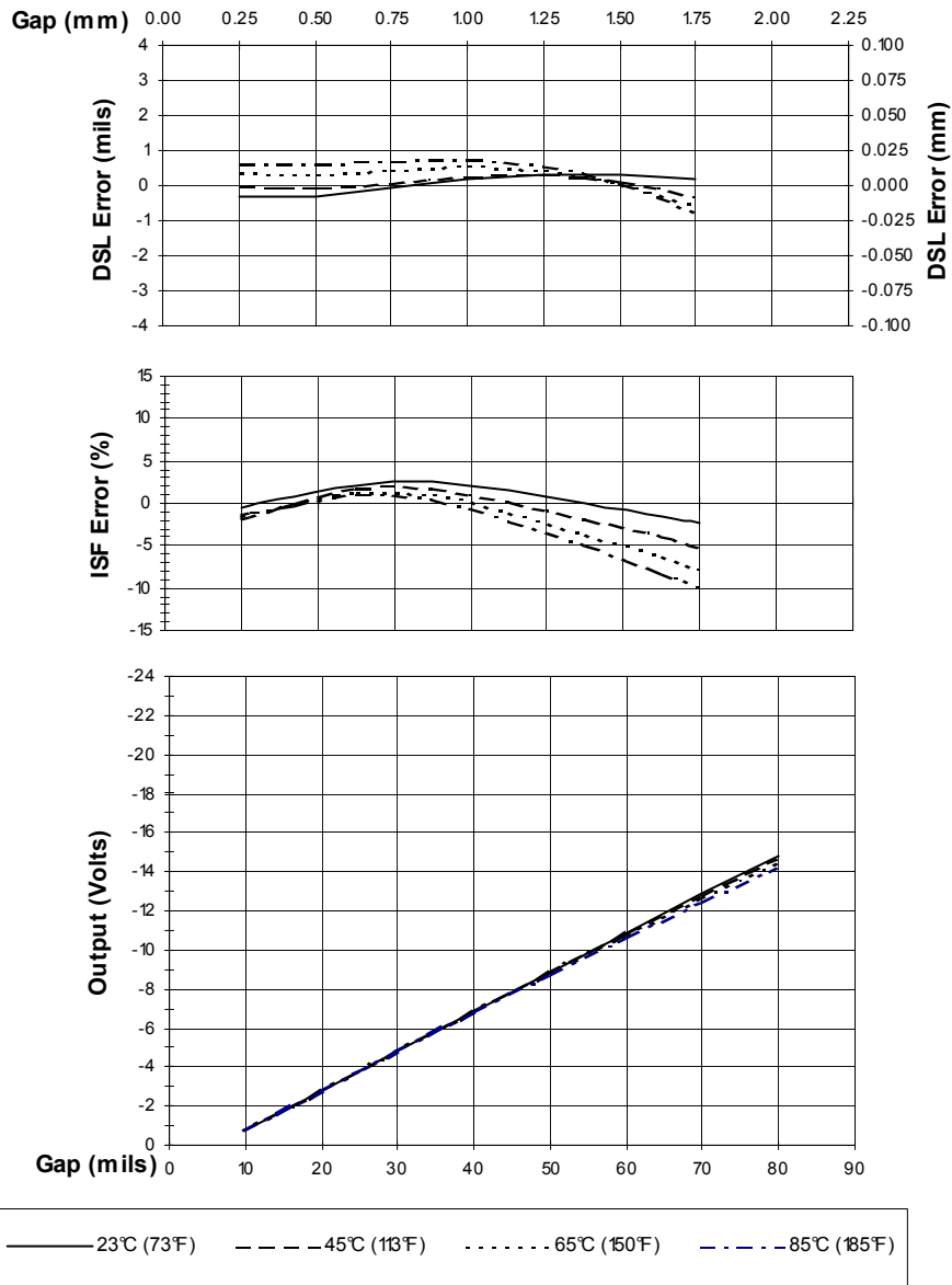
Figure 8 Typical 3300 XL NSv™ 7 m Proximator® Sensor with 6 m of Extension Cable @ High Temperature (Probe is at 25°C)
