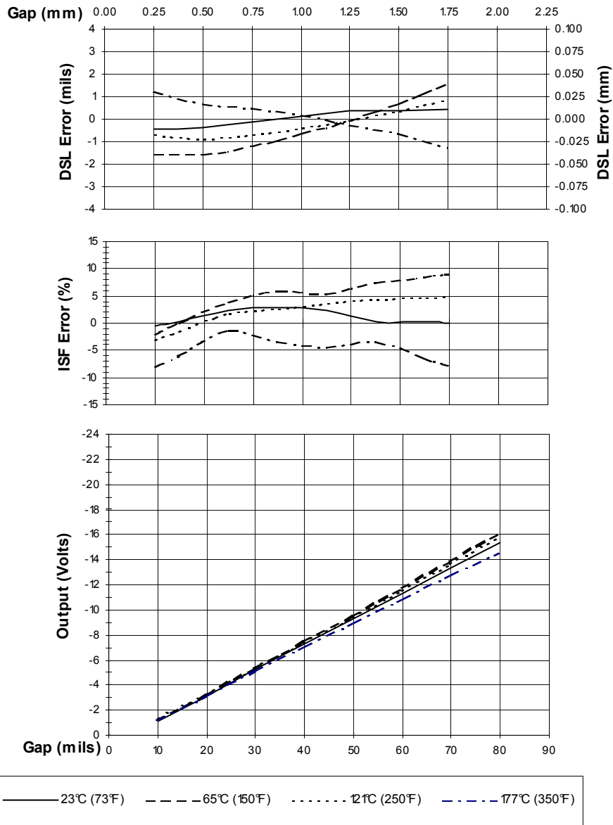
Figure 4 Typical 3300 NSv™ Probe + 1m Cable @ High Temperature (Proximitytor® Sensor + 4m of Extension Cable @ 25 °C)
