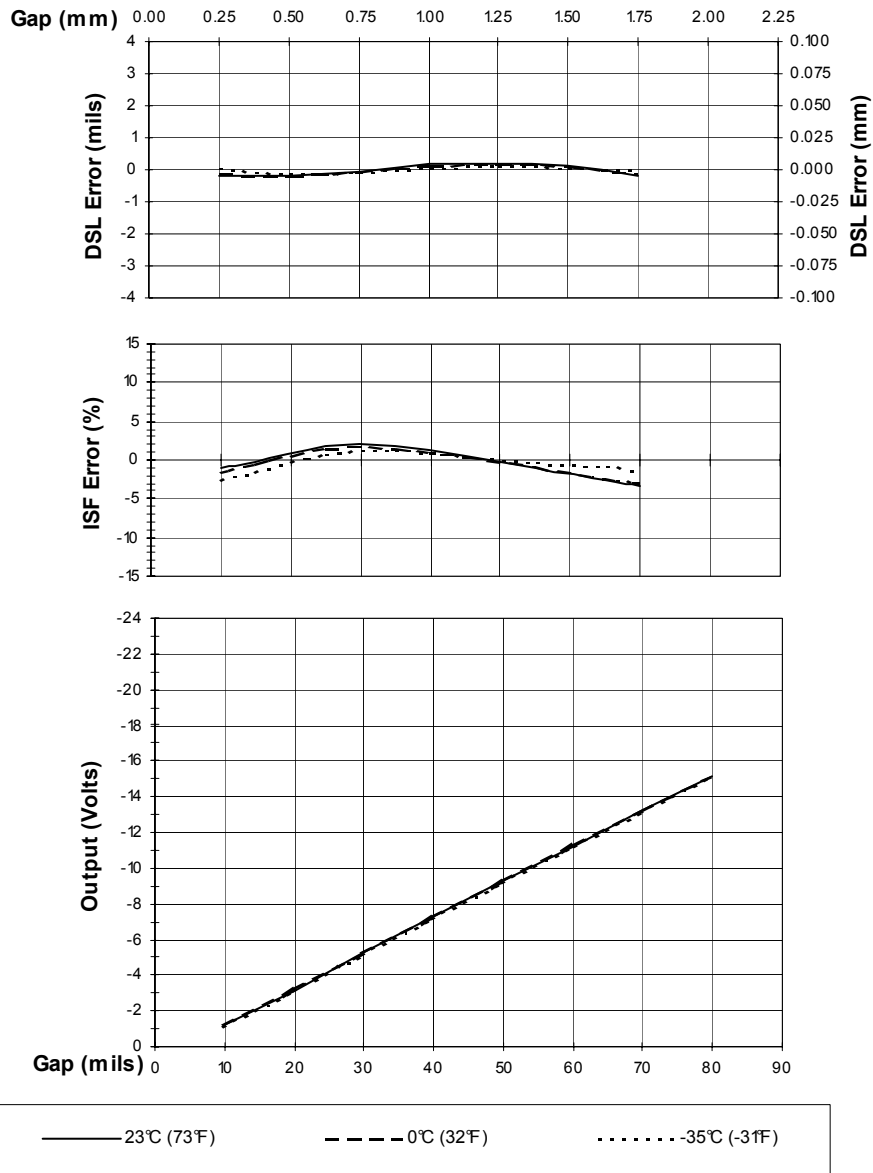
Figure 7 Typical 3300 XL NSv™ 7 m Proximator® Sensor with 6 m of Extension Cable @ Low Temperature (Probe is at 25°C)
