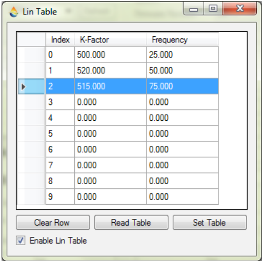
Figure 15: Linearizer Table
