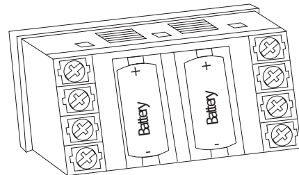
Figure 2: Battery installation
