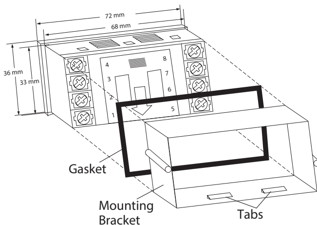
Figure 1: Panel installation
