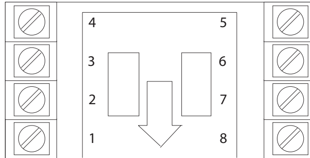
Figure 3: Wiring terminals
