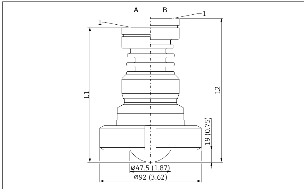
29 Dimensions of antenna, cladded flush mount, PTFE, 50 mm (2 in), slotted nut DIN11851. Unit of measurement mm (in)
