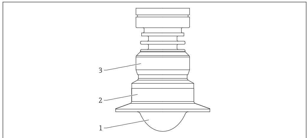
37 Material; antenna, cladded flush mount, PTFE, 50 mm (2 in), with Tri-Clamp ISO2852. Unit of measurement mm (in)
