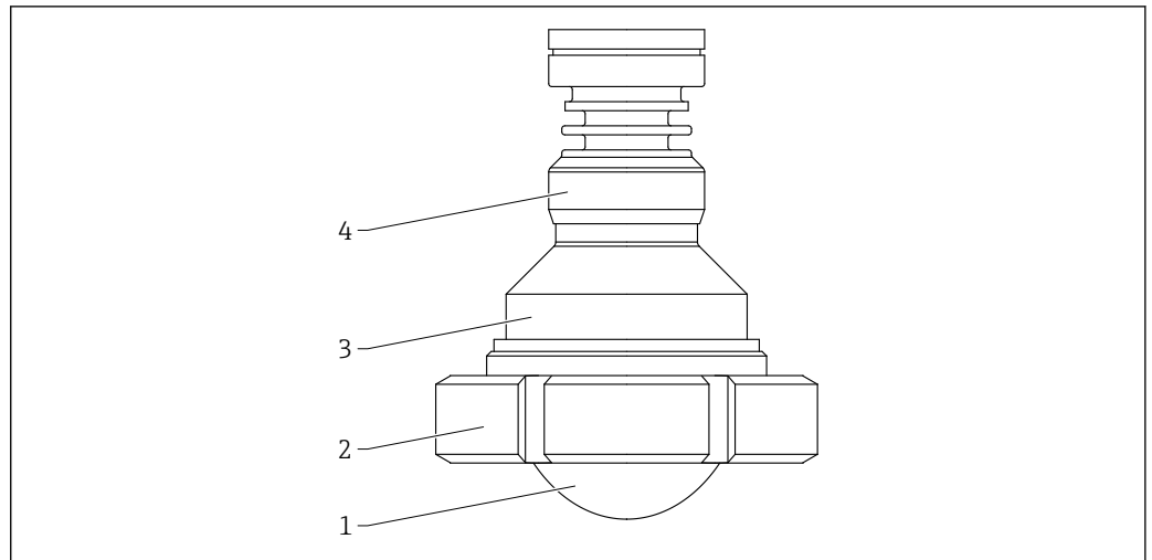
36 Material; antenna, cladded flush mount, 80 mm (3 in), slotted nut DIN11851. Unit of measurement mm (in)
