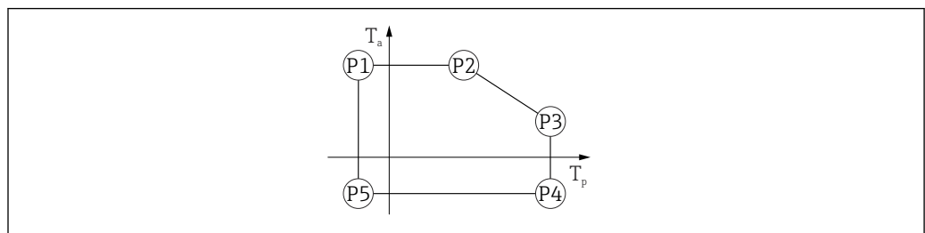
18 Aluminum housing material; process temperature range: -40 to +150 °C (-40 to +302 °F)
