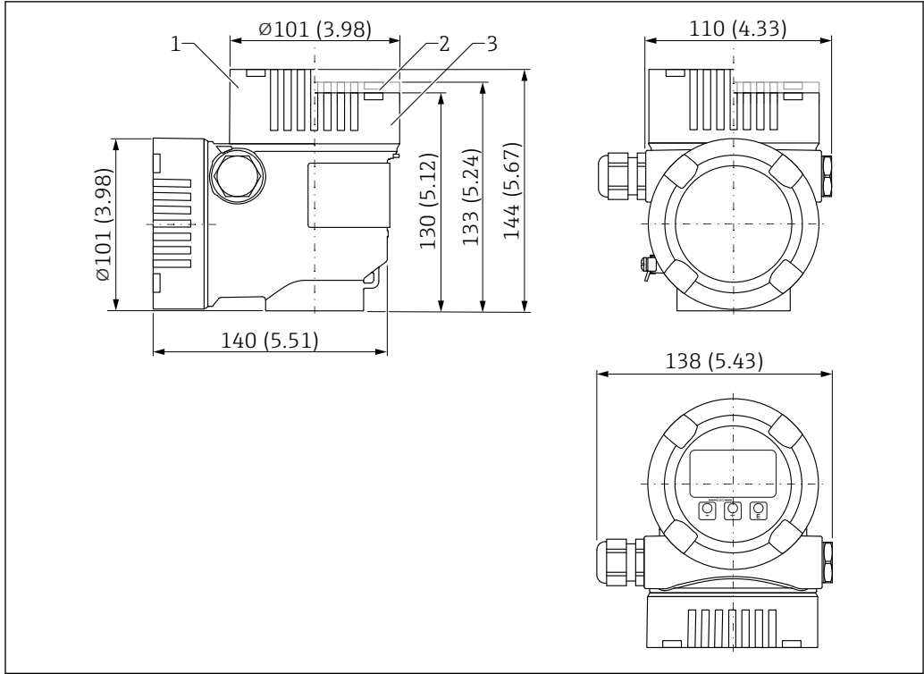
27 Dimensions of dual compartment housing, L-form 1 Height with cover with glass viewing window (devices for Ex d, dust Ex) 2 Height with cover with plastic viewing window 3 Cover without viewing window
