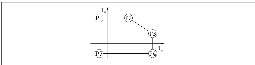
12 Plastic housing material; process temperature range: -40 to +150 °C ( -40 to +302 °F)
