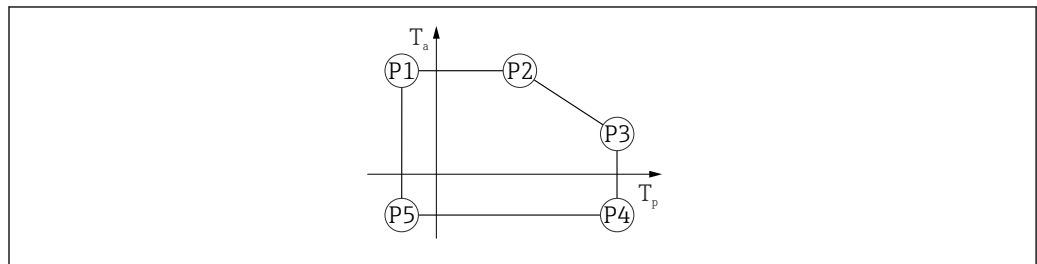
17 Aluminum housing material; process temperature range: -20 to +200 °C (-4 to +392 °F)
