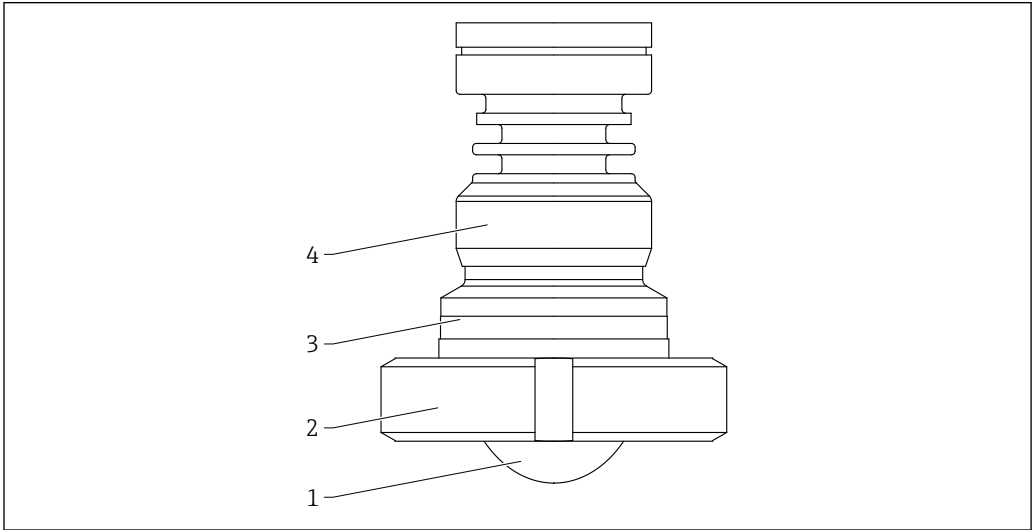
35 Material; antenna, cladded flush mount, 50 mm (2 in), slotted nut DIN11851
