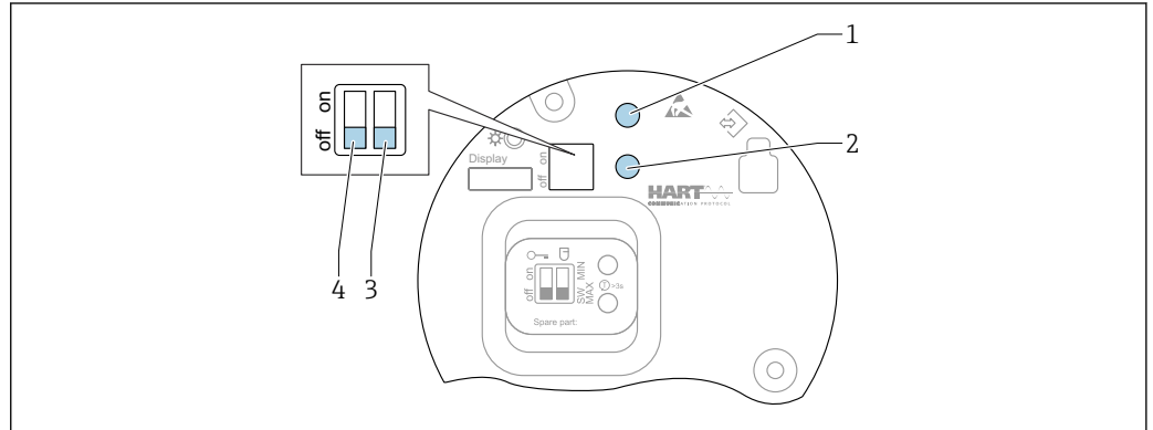
39 Operating keys and DIP switches on the HART electronic insert
