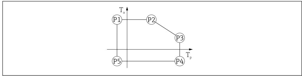
16 Aluminum housing material; process temperature range: -20 to +150 °C (-4 to +302 °F)
