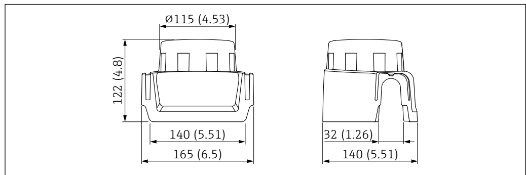
42 Dimensions. Unit of measurement mm (in)
