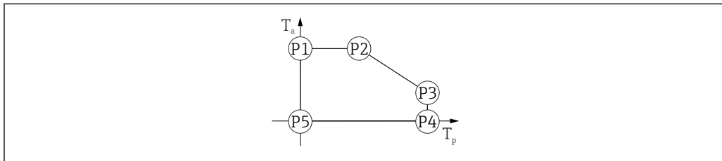
11 Plastic housing material; process temperature range: 0 to +200 °C ( +32 to +392 °F) with CSA C/US approval
