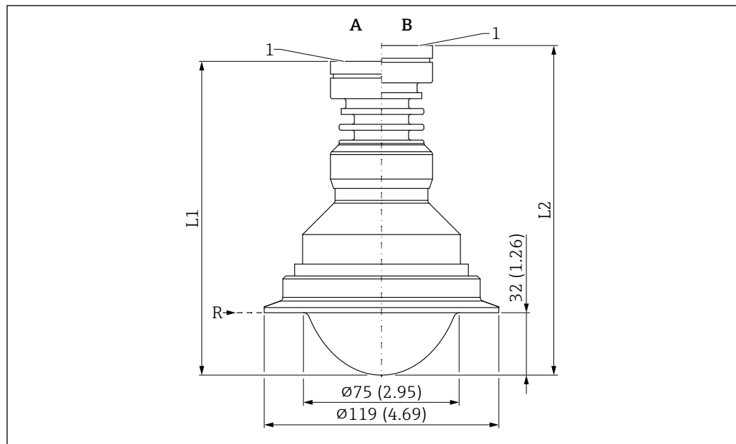
33 Dimensions of antenna, cladded flush mount, PTFE, 80 mm (3 in), with Tri-Clamp DN101.6 (4") ISO2852. Unit of measurement mm (in)
