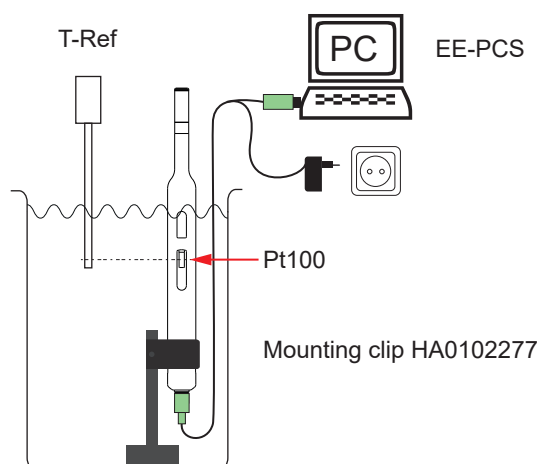
Fig. 7 Temperature calibration/adjustment in a liquid bath
