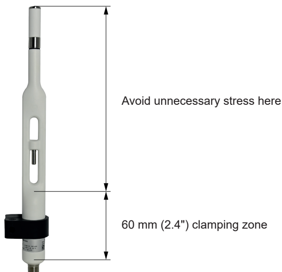
Fig. 4 EE260 mounted with the optional clip HA010227
