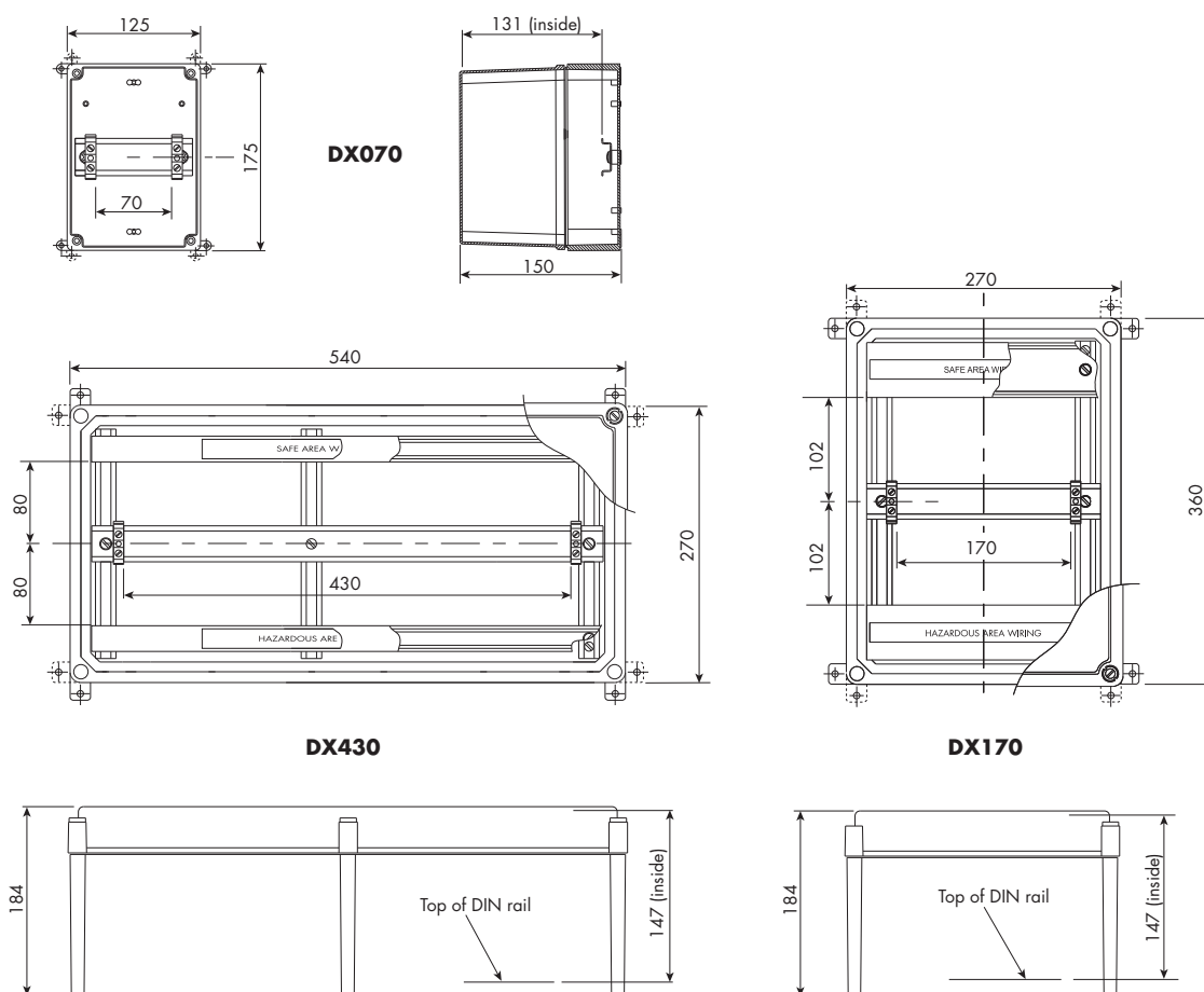
Figure 5.1: MTL's DX range of enclosures
