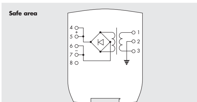
Figure 6.80: MTL5991 wiring diagram and connections
