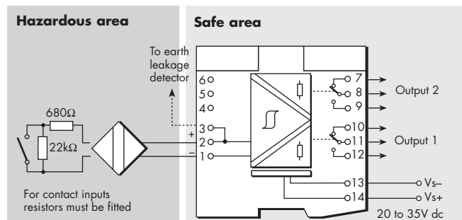
Figure 6.7: MTL5014 wiring diagram and connections
