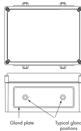
Figure 5.10: Cable gland plate locations on a DX170 enclosure
