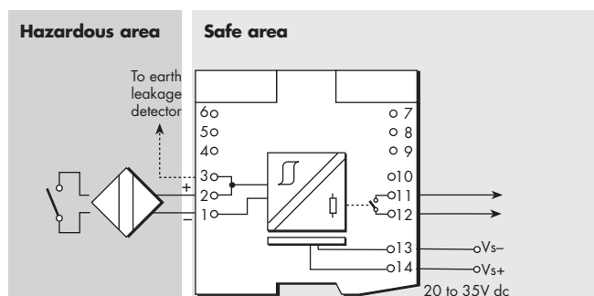
Figure 6.1: MTL5011 wiring diagram and connections
