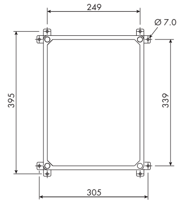
Figure 5.8: Dimensions and location of fixing holes - DX170
