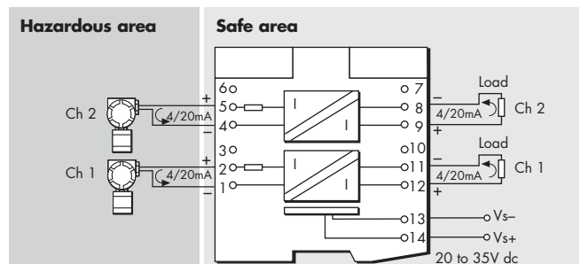
Figure 6.43: MTL5044 wiring diagram and connections
