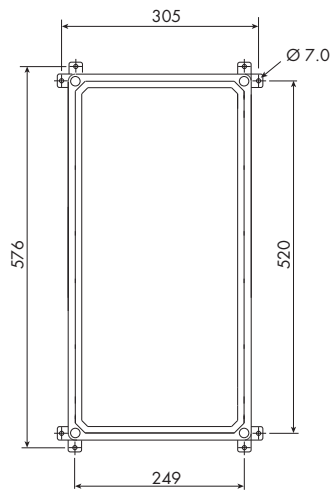
Figure 5.9: Dimensions and location of fixing holes - DX430
