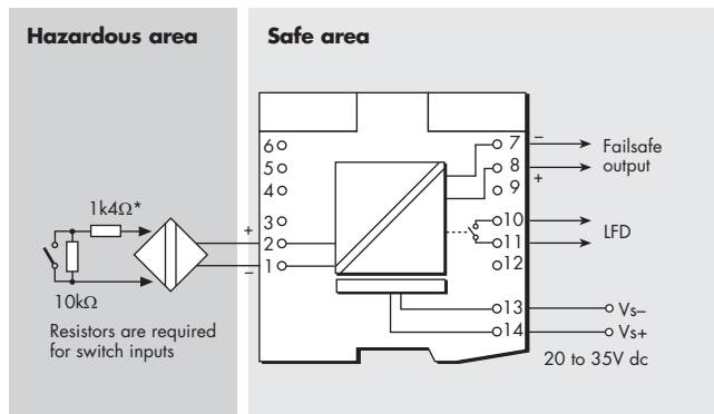
Figure 6.71: MTL5113P wiring diagram and connections
