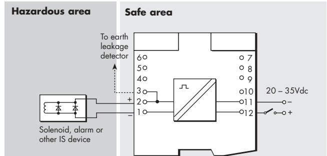
Figure 6.20: MTL5021 wiring diagram and connections
