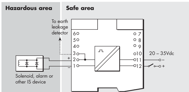
Figure 6.22: MTL5022 wiring diagram and connections
