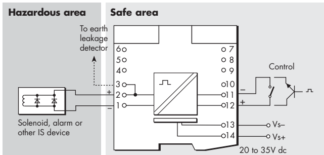
Figure 6.26: MTL5024 wiring diagram and connections
