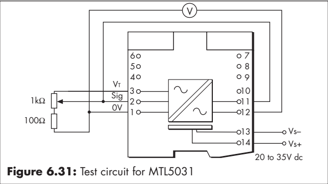
Figure 6.31: Test circuit for MTL5031 Measure the voltage on terminal 3 with respect to terminal 1; this should be >19V. Vary the potentiometer setting and check that the reading on voltmeter V varies by no more than ±100mV.
