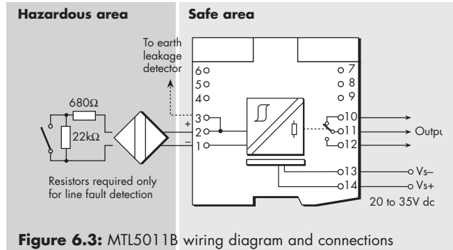
Figure 6.3: MTL5011B wiring diagram and connections
