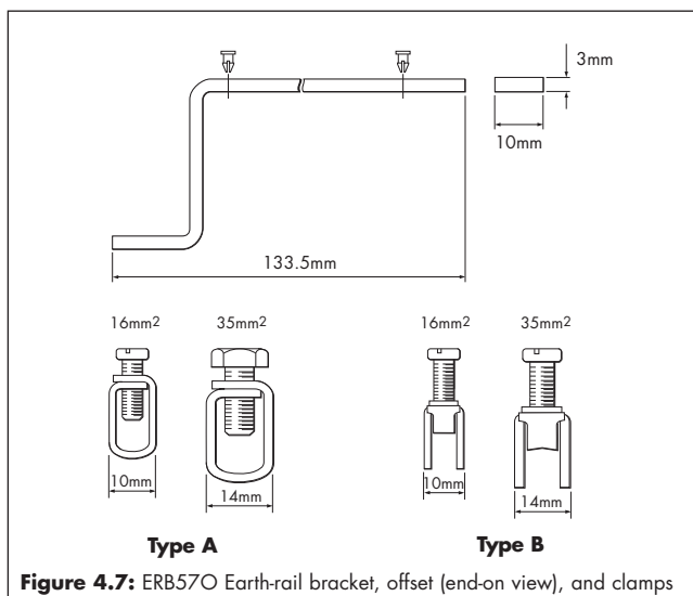
Figure 4.7: ERB57O Earth-rail bracket, offset (end-on view), and clamps
