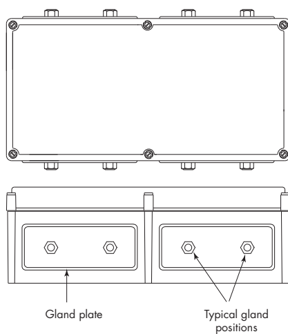
Figure 5.11: Cable gland plate locations on a DX430 enclosure
