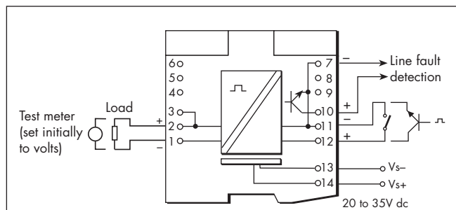
Figure 6.25: Test circuit for MTL5023
