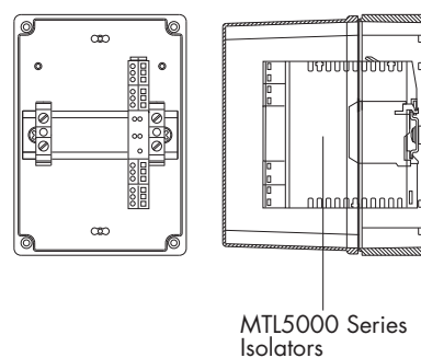
Figure 5.2: DX070 enclosure showing MTL5000 modules mounted
