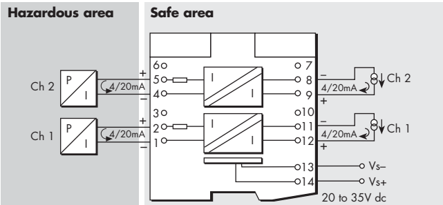
Figure 6.78: MTL5349 wiring diagram and connections
