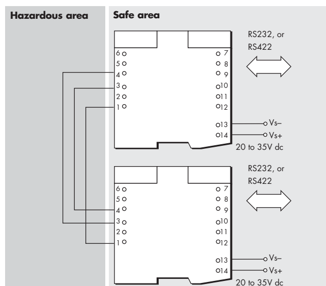
Figure 6.53: MTL5051 wiring diagram (across a hazardous area)
