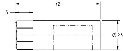
HIGH PRESSURE CONSTRUCTION (ALL RANGES: > 70 bar TO \leq 700 bar)
