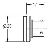
BAYONET MIL-C-26482
