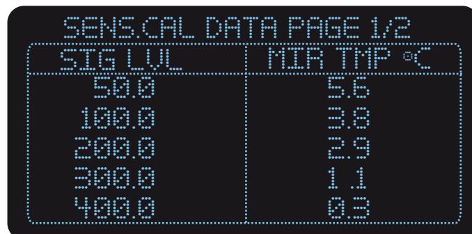
Figure 25 Sensitivity Calibration Data Page
