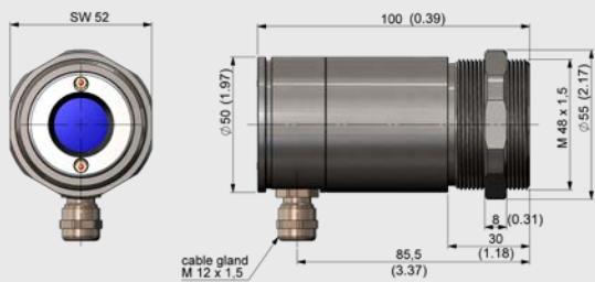
Sensing head
