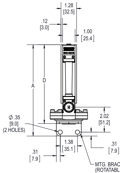
REGULATING VALVE
